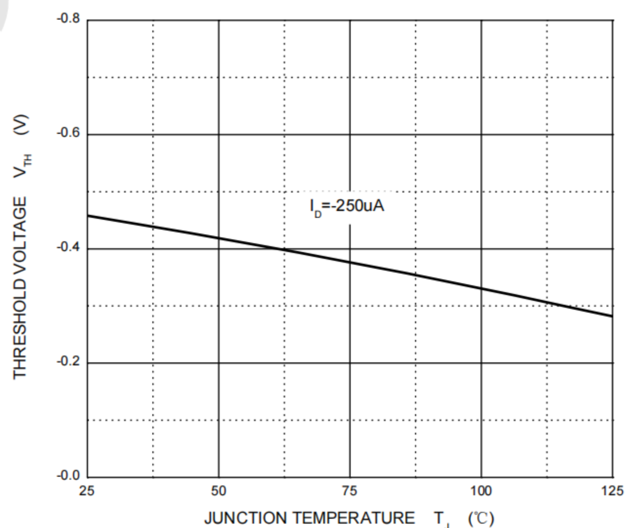
Threshold Voltage
