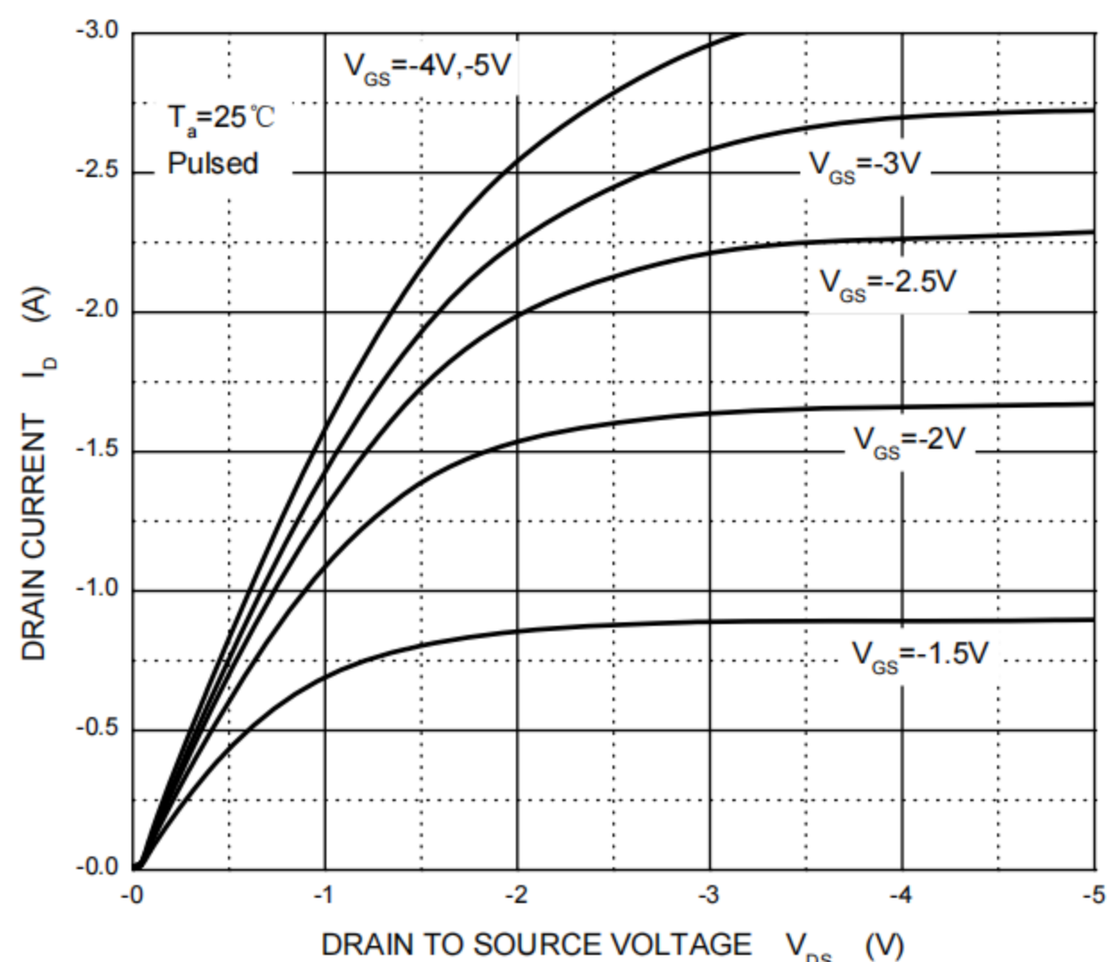
Output Characteristics
