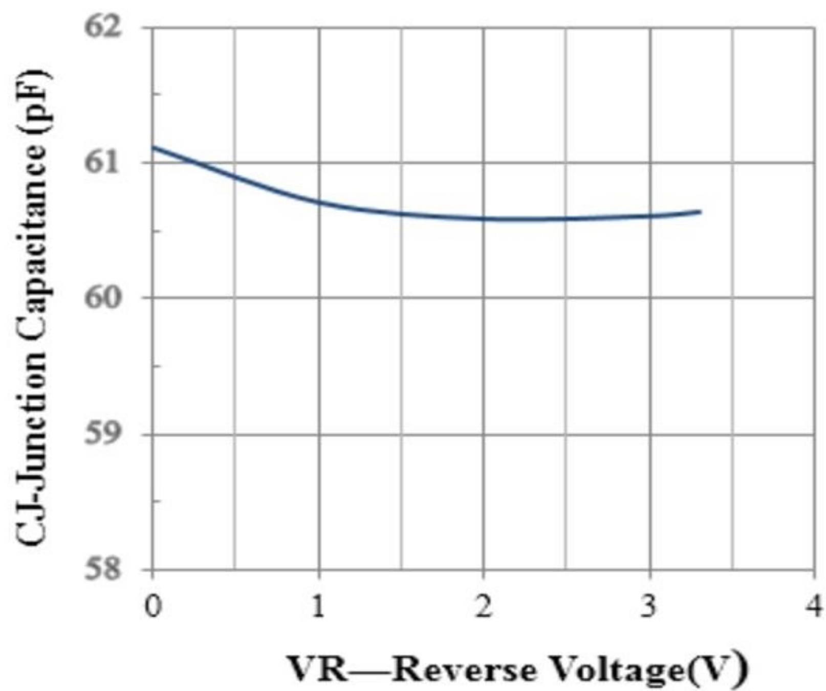
Junction Capacitance vs. Reverse Voltage
