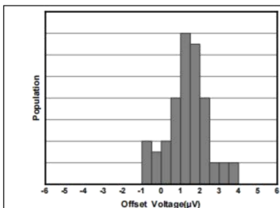
Figure 2. Offset Voltage Production Distribution
